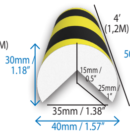
Round Corner Bumper Part #: RCB120 Quantity / Pack: 1
