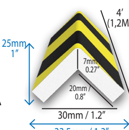
Square Corner Bumper Part #: SCB120 Quantity / Pack: 1
