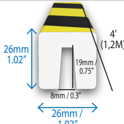
Square I-Beam Protector Part #: SIBP120 Quantity / Pack: 1
